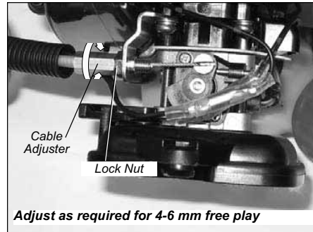
Throttle Lever Free Play
